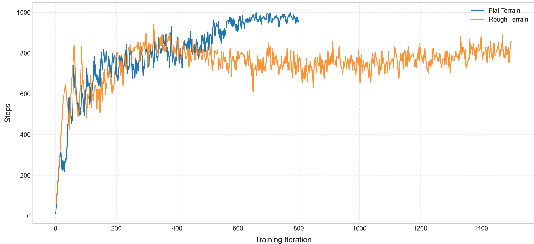
Mean Episode Length
